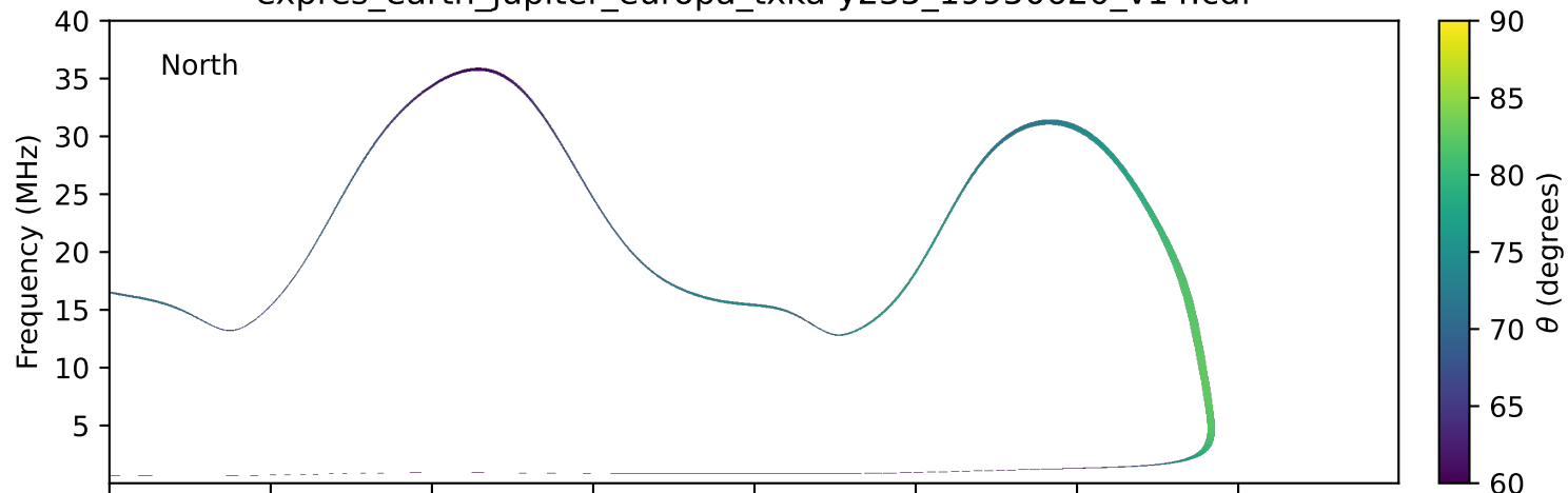
expres_earth_jupiter_europa_txka-y235_19950620_v14.cdf
