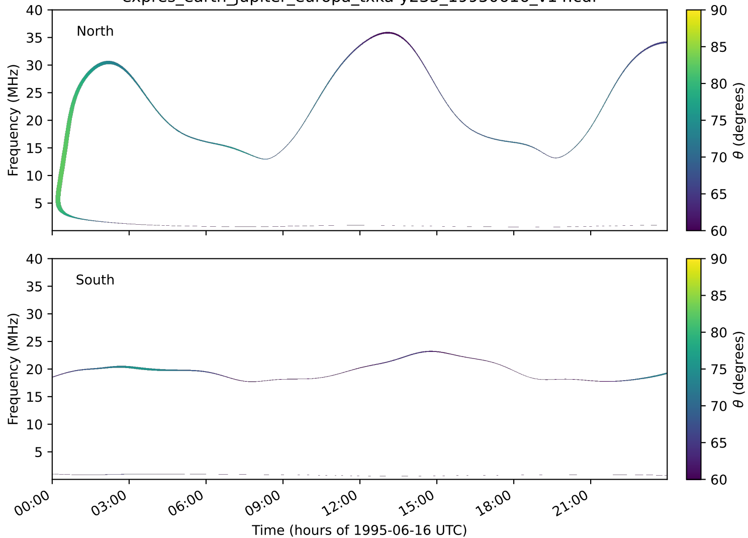
expres_earth_jupiter_europa_txka-y235_19950616_v14.cdf
