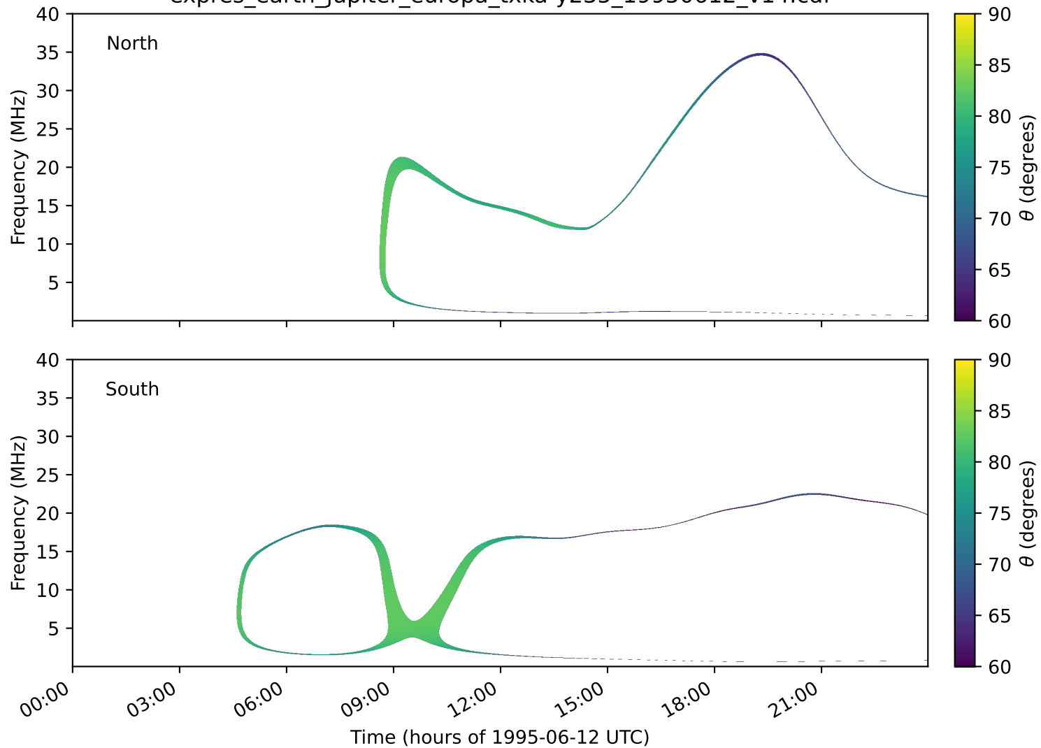
expres_earth_jupiter_europa_txka-y235_19950612_v14.cdf
