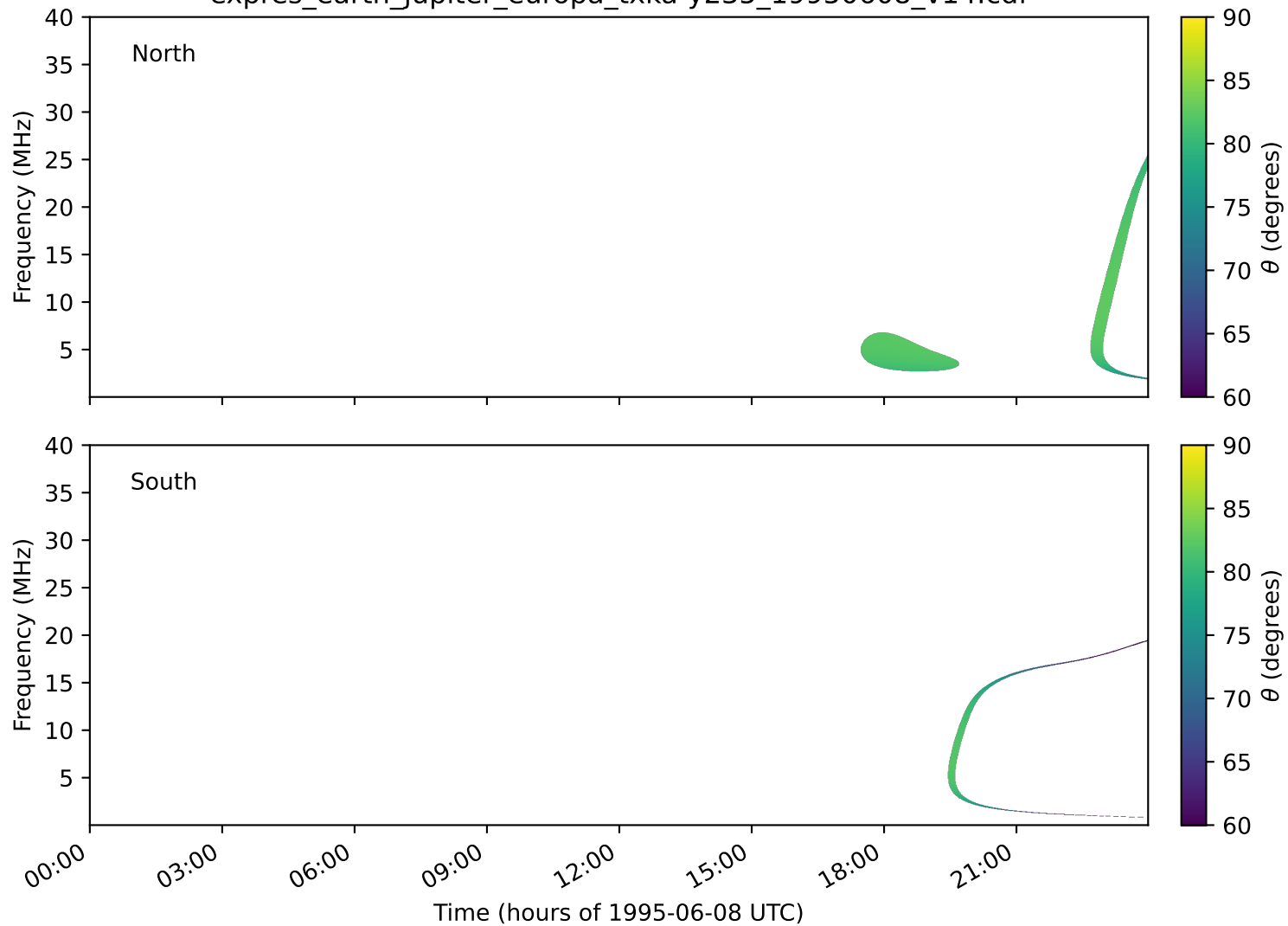
expres_earth_jupiter_europa_txka-y235_19950608_v14.cdf
