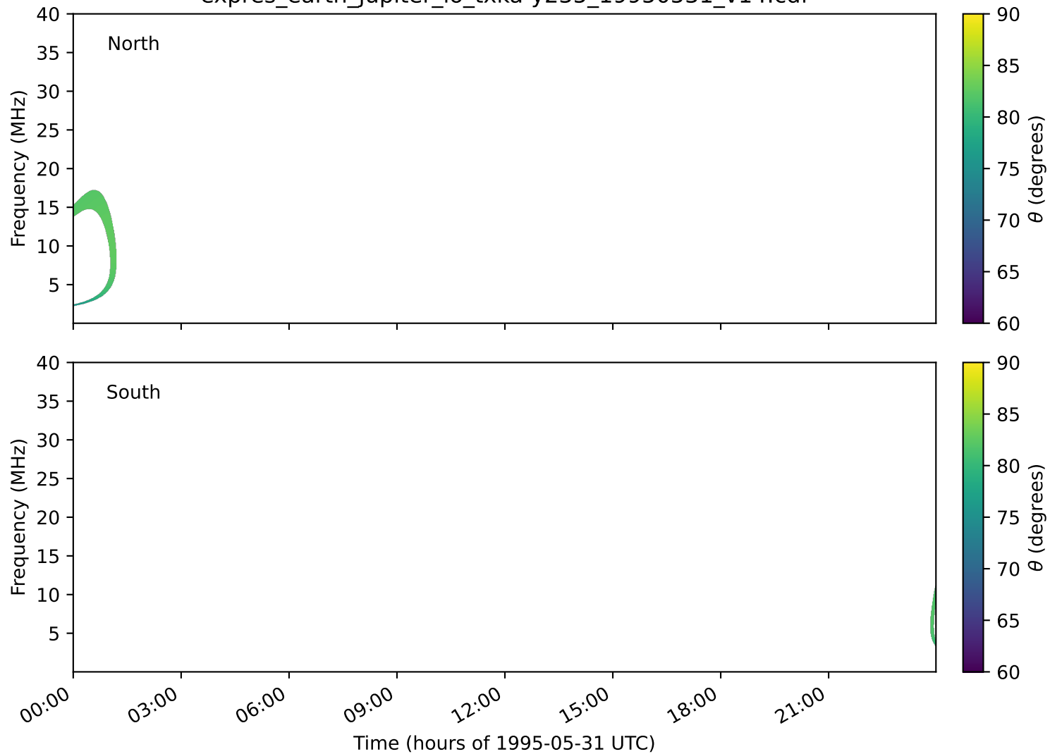
expres_earth_jupiter_io_txka-y235_19950531_v14.cdf
