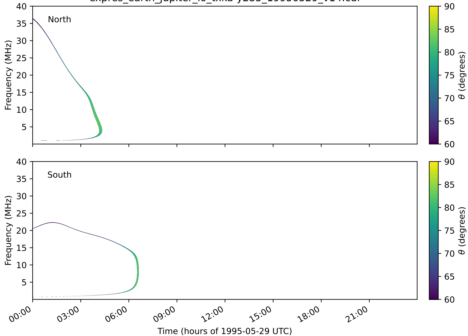
expres_earth_jupiter_io_txka-y235_19950529_v14.cdf
