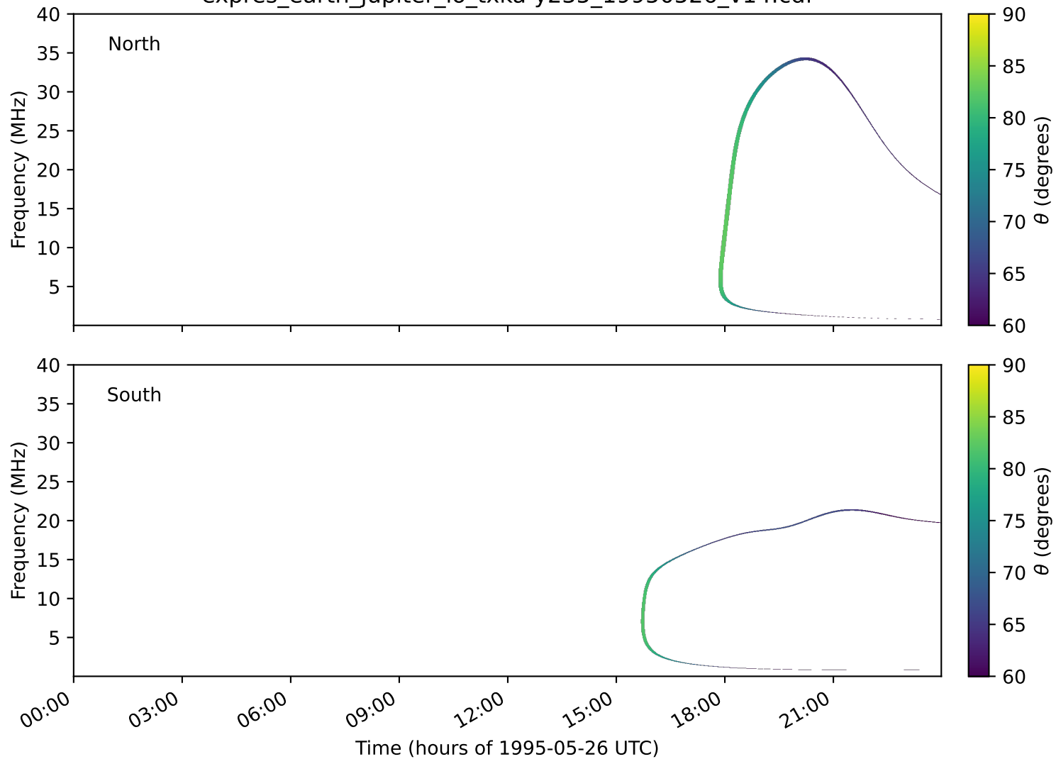
expres_earth_jupiter_io_txka-y235_19950526_v14.cdf
