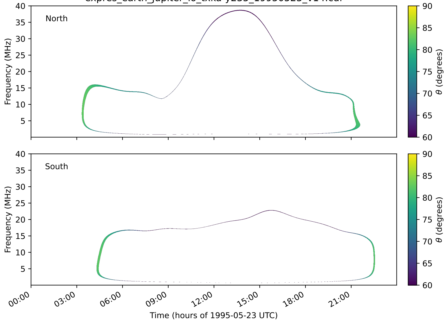
expres_earth_jupiter_io_txka-y235_19950523_v14.cdf
