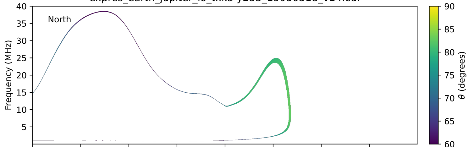
expres_earth_jupiter_io_txka-y235_19950518_v14.cdf
