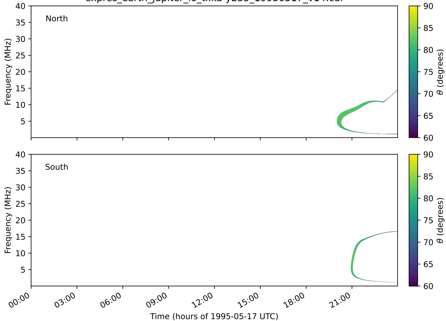
expres_earth_jupiter_io_txka-y235_19950517_v14.cdf
