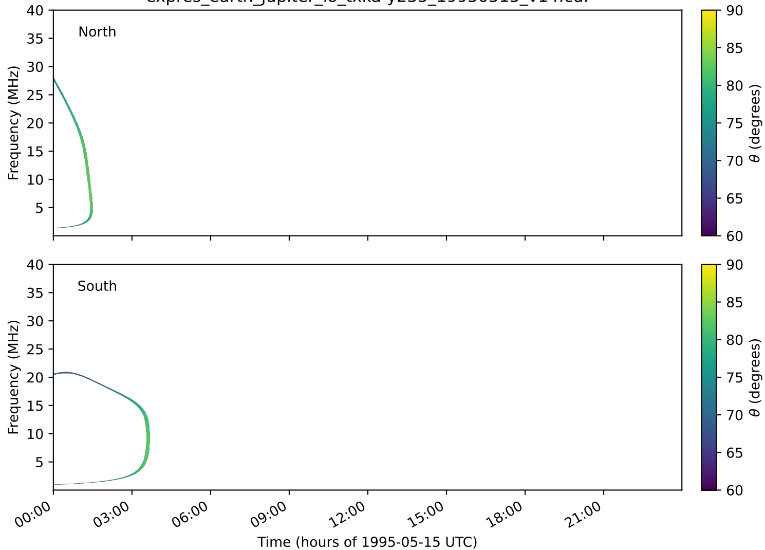
expres_earth_jupiter_io_txka-y235_19950515_v14.cdf
