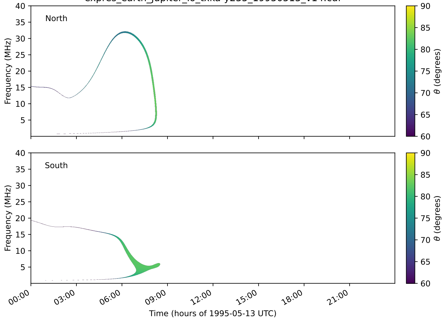
expres_earth_jupiter_io_txka-y235_19950513_v14.cdf
