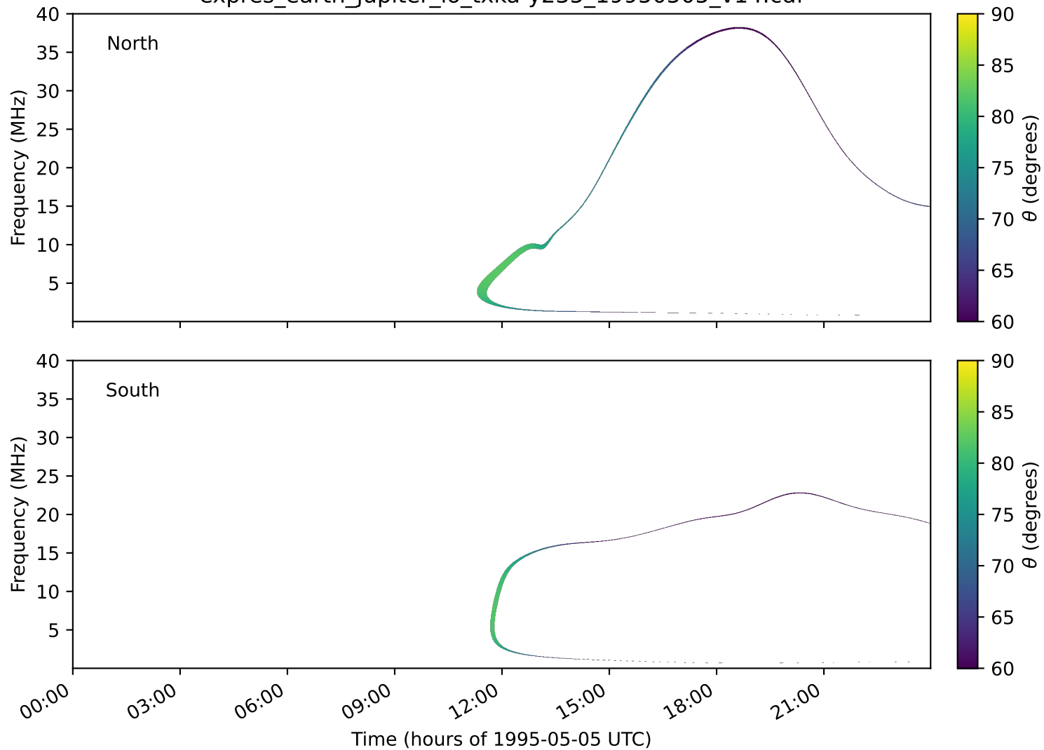
expres_earth_jupiter_io_txka-y235_19950505_v14.cdf
