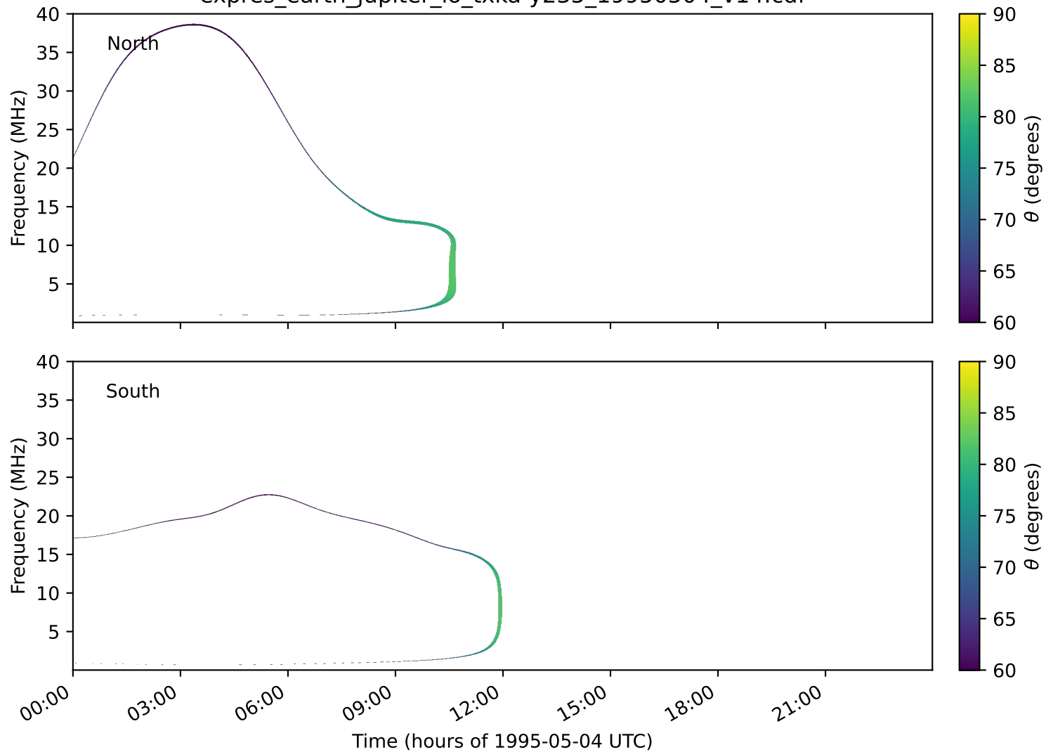
expres_earth_jupiter_io_txka-y235_19950504_v14.cdf
