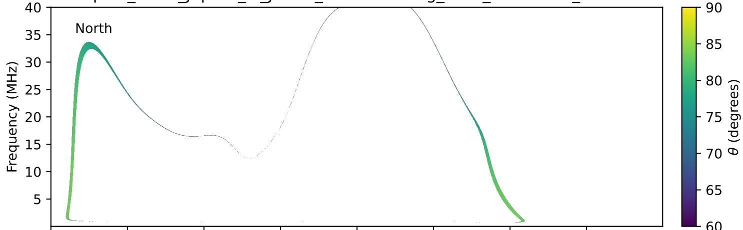
expres_earth_jupiter_io_jrm33_lossc-wid1deg_3kev_19950509_v11.cdf
