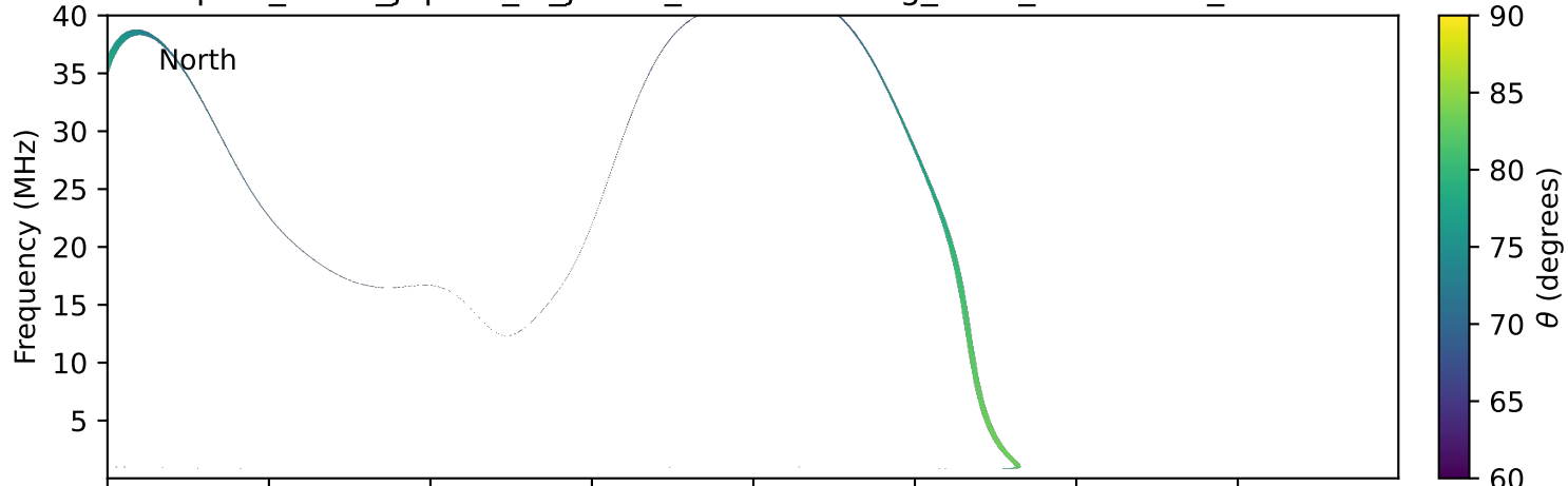
expres_earth_jupiter_io_jrm33_lossc-wid1deg_3kev_19950502_v11.cdf
