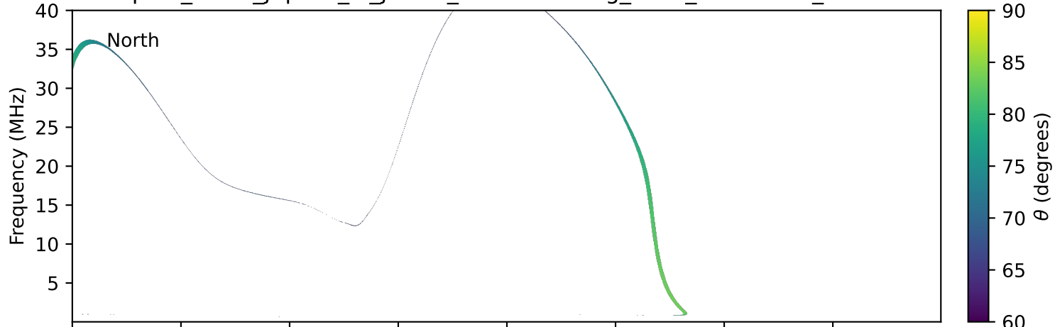
expres_earth_jupiter_io_jrm09_lossc-wid1deg_3kev_19950502_v11.cdf
