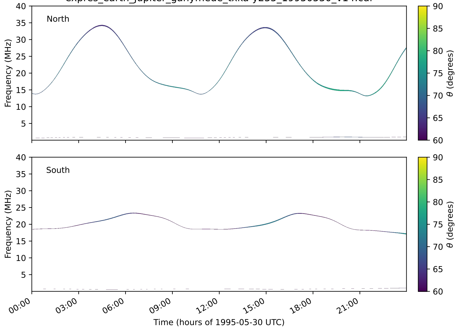
expres_earth_jupiter_ganymede_txka-y235_19950530_v14.cdf
