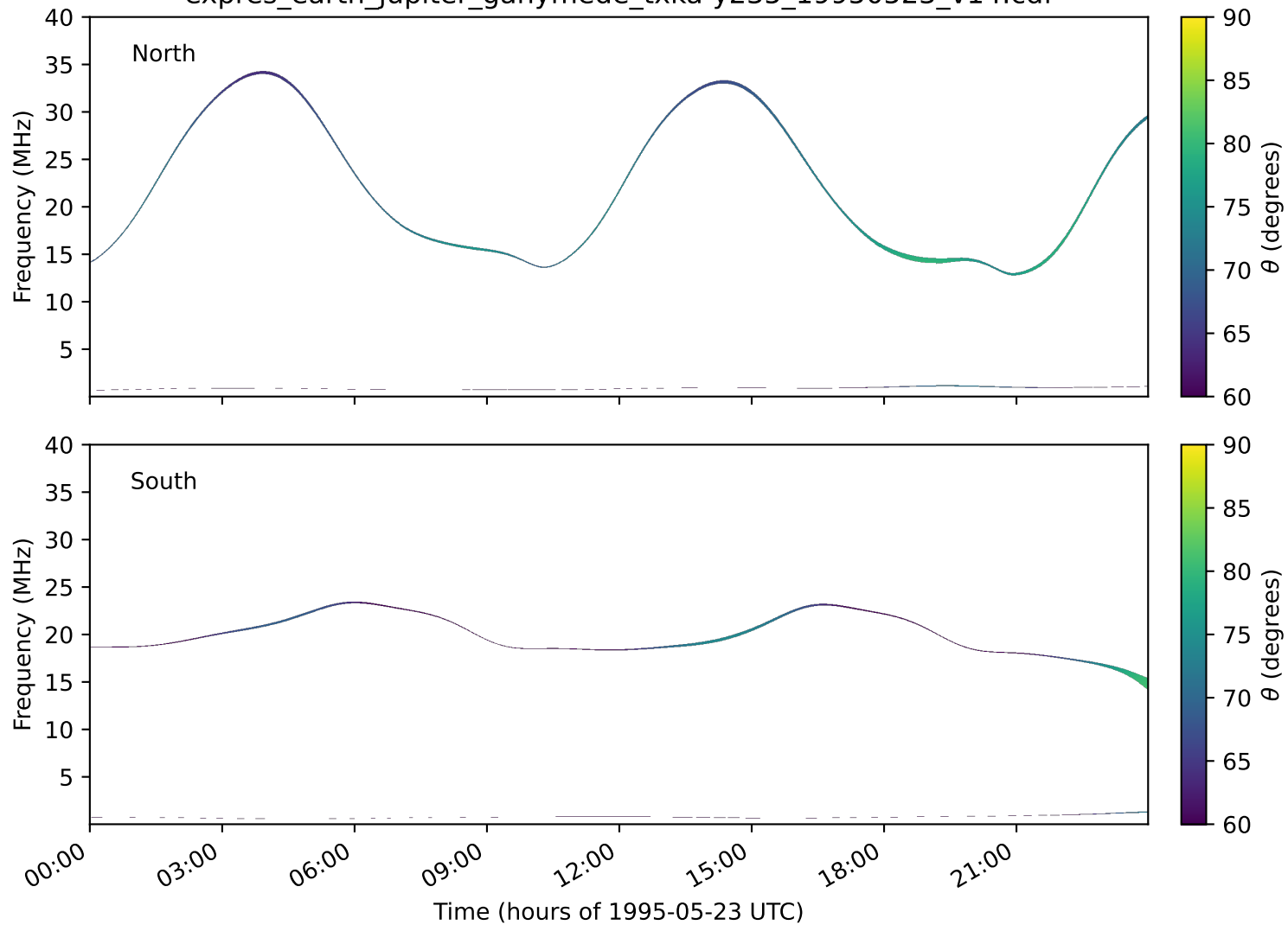
expres_earth_jupiter_ganymede_txka-y235_19950523_v14.cdf
