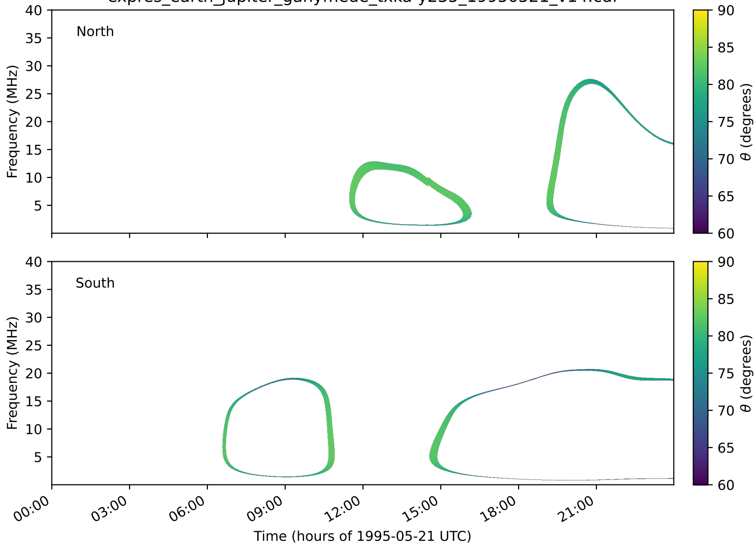
expres_earth_jupiter_ganymede_txka-y235_19950521_v14.cdf
