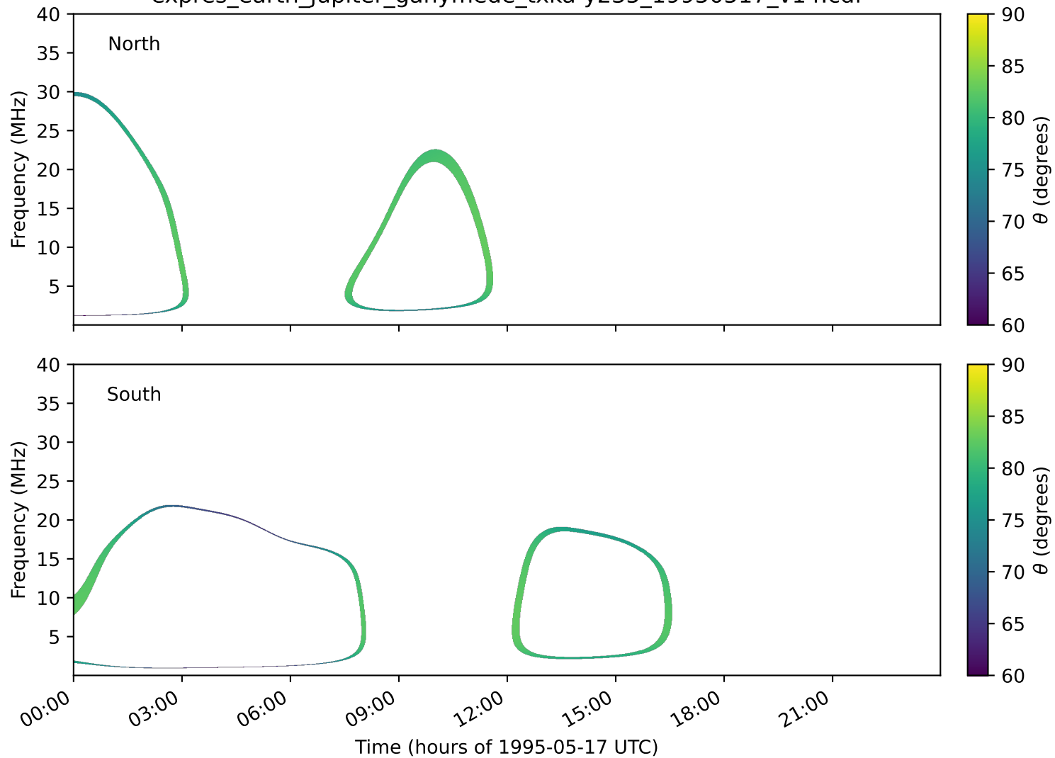
expres_earth_jupiter_ganymede_txka-y235_19950517_v14.cdf
