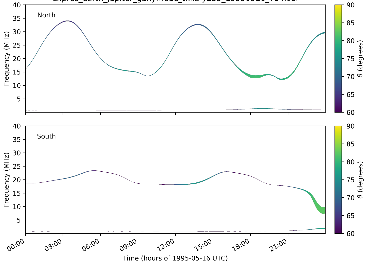
expres_earth_jupiter_ganymede_txka-y235_19950516_v14.cdf
