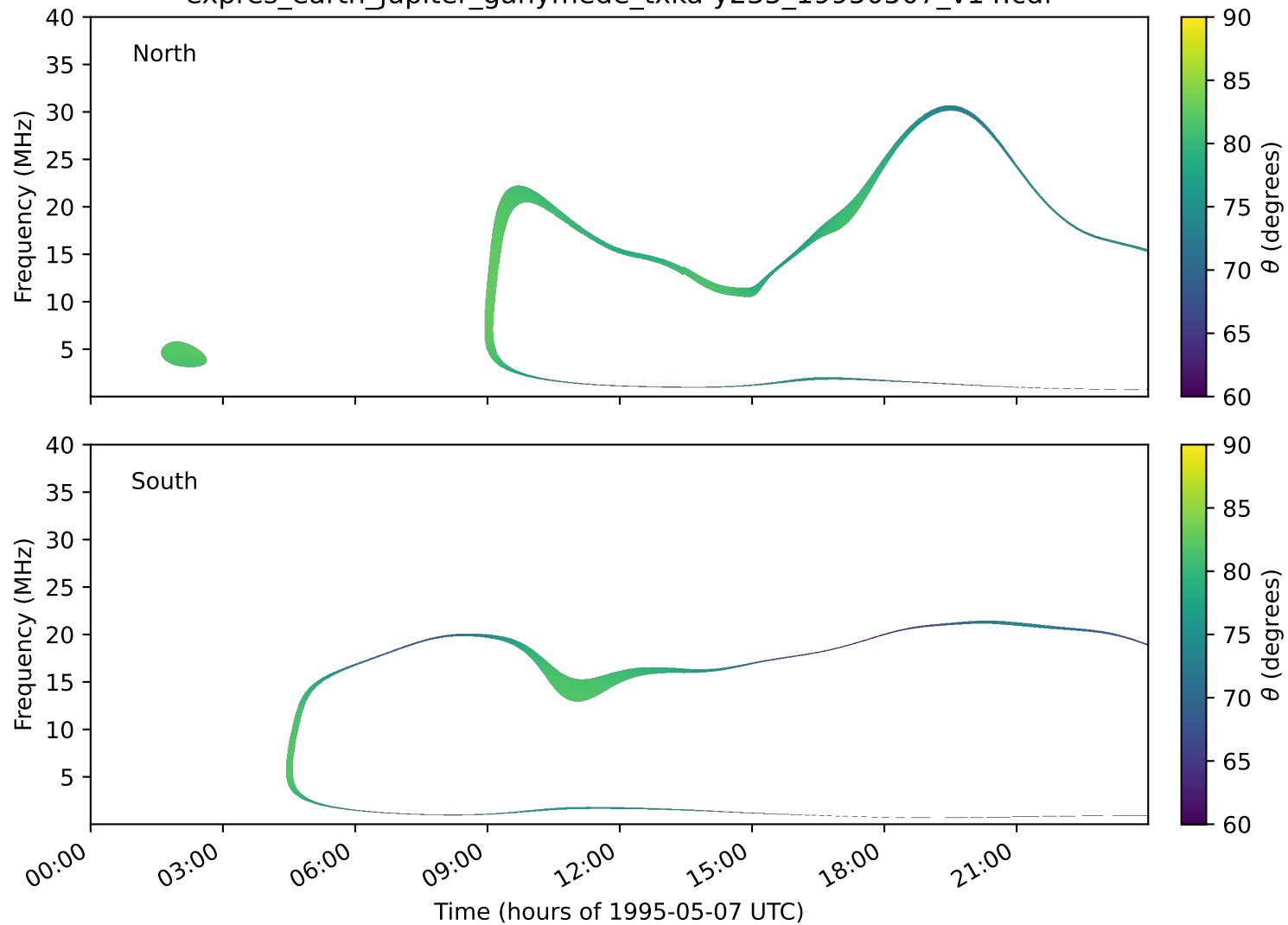
expres_earth_jupiter_ganymede_txka-y235_19950507_v14.cdf
