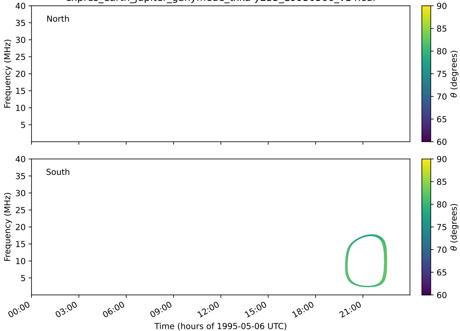
expres_earth_jupiter_ganymede_txka-y235_19950506_v14.cdf
