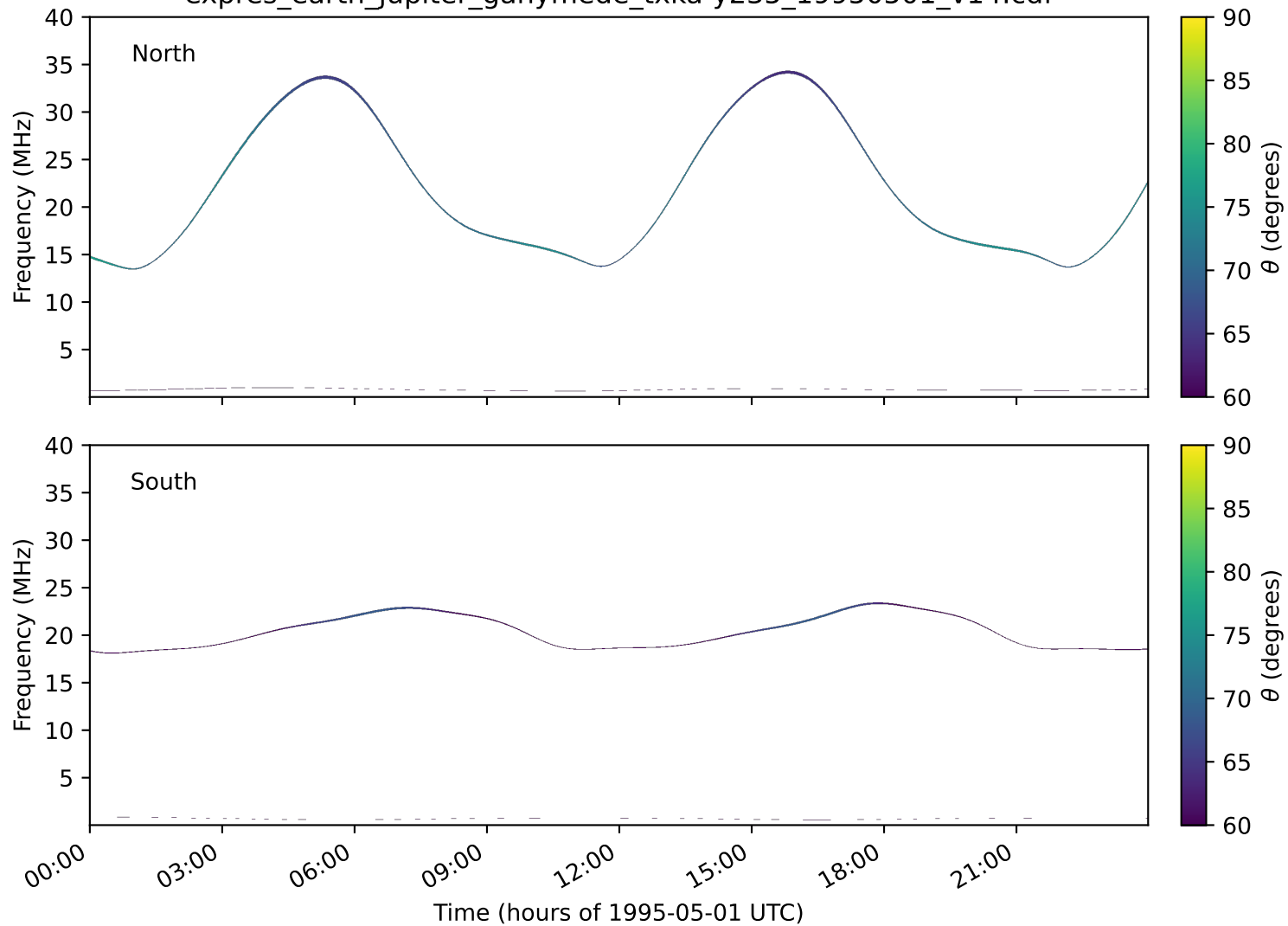
expres_earth_jupiter_ganymede_txka-y235_19950501_v14.cdf
