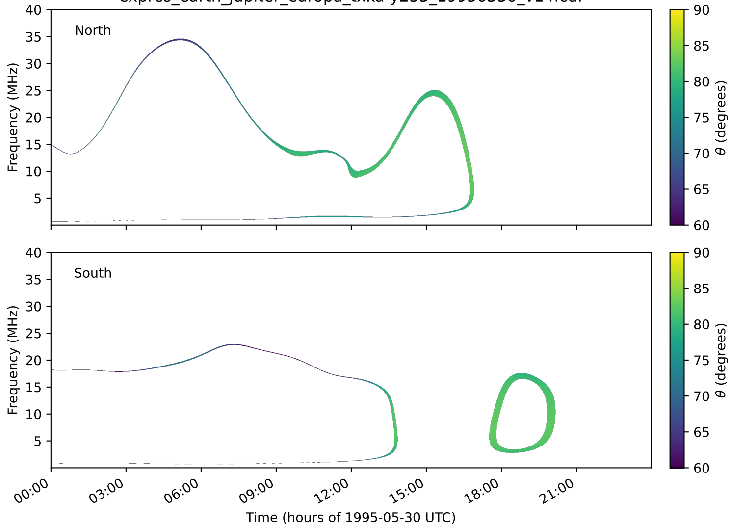
expres_earth_jupiter_europa_txka-y235_19950530_v14.cdf
