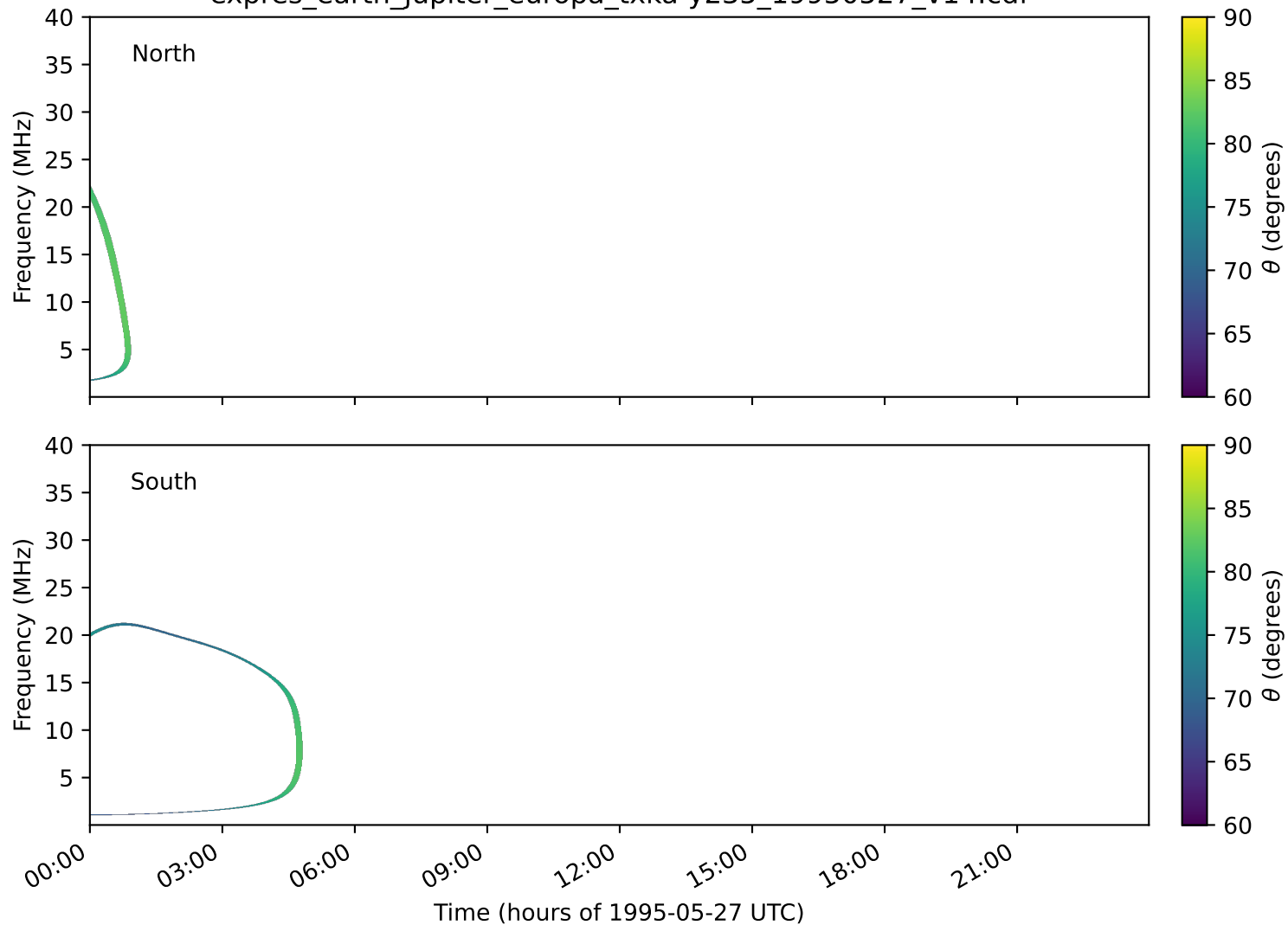
expres_earth_jupiter_europa_txka-y235_19950527_v14.cdf
