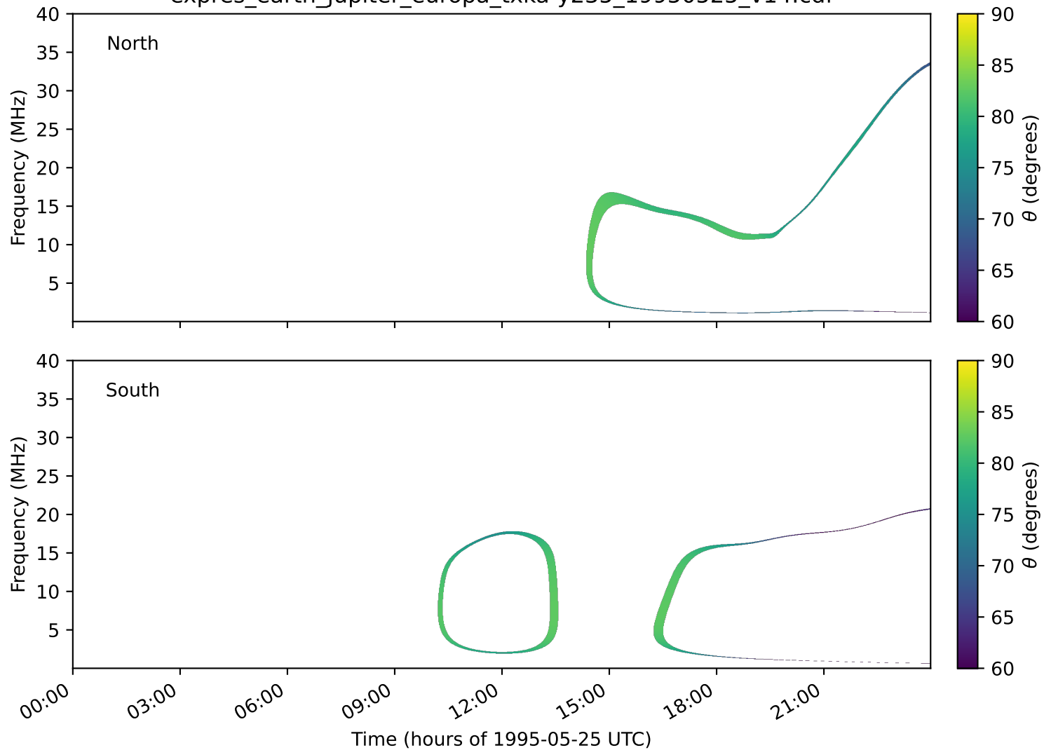
expres_earth_jupiter_europa_txka-y235_19950525_v14.cdf
