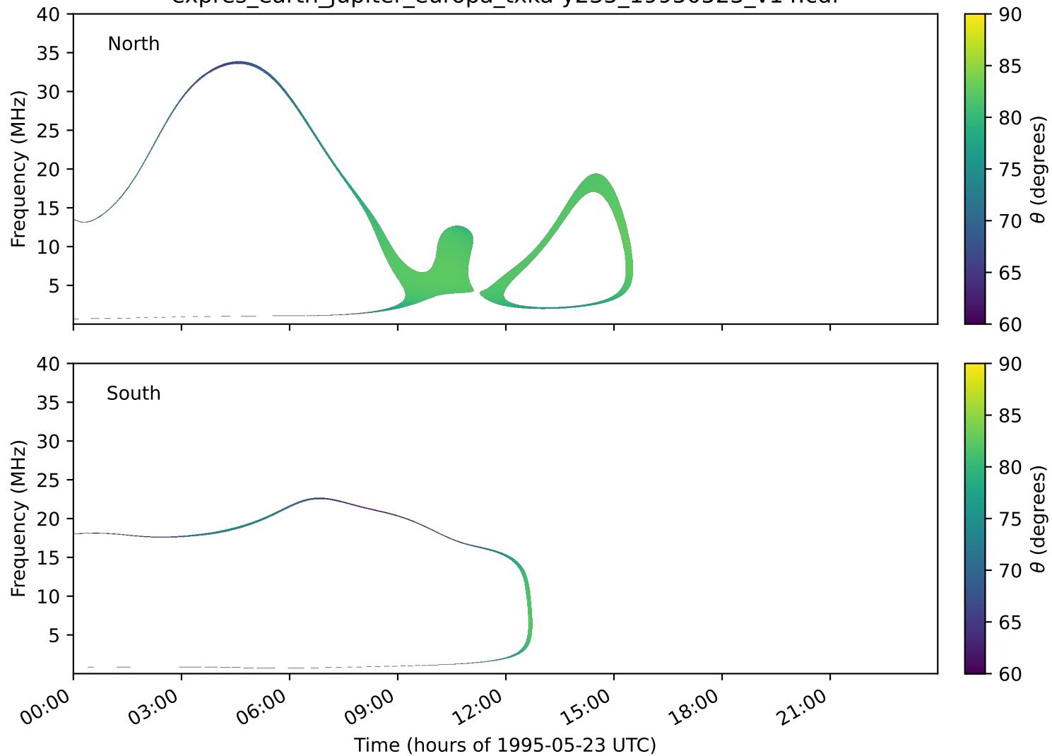
expres_earth_jupiter_europa_txka-y235_19950523_v14.cdf
