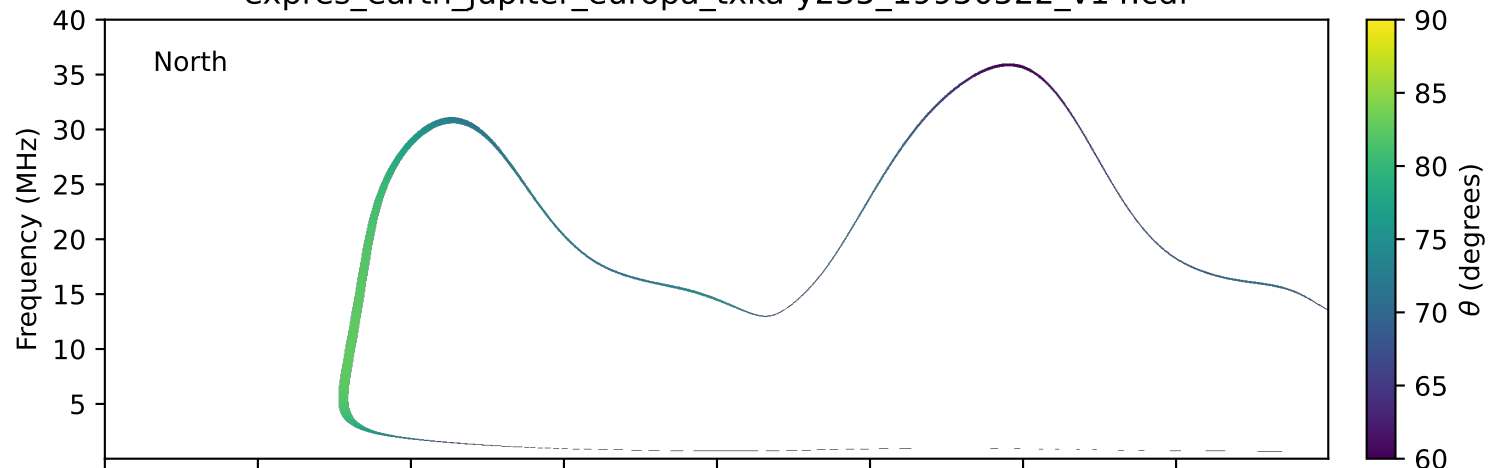
expres_earth_jupiter_europa_txka-y235_19950522_v14.cdf
