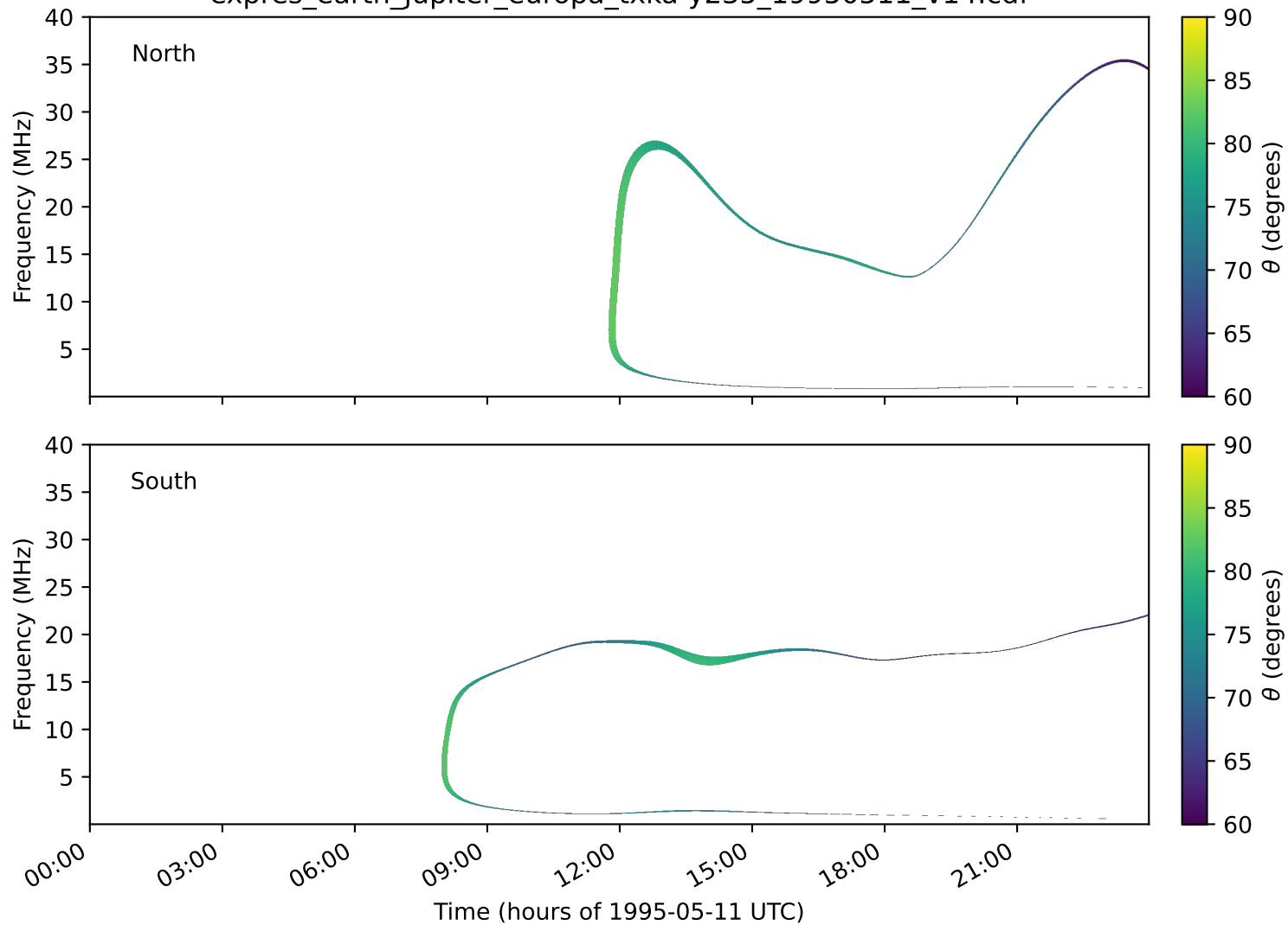
expres_earth_jupiter_europa_txka-y235_19950511_v14.cdf
