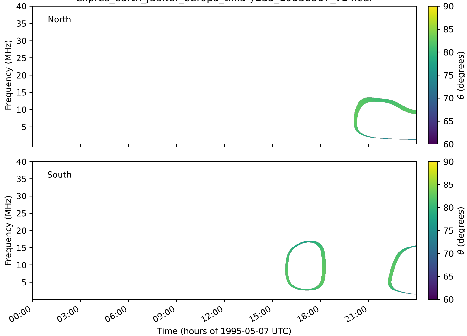
expres_earth_jupiter_europa_txka-y235_19950507_v14.cdf
