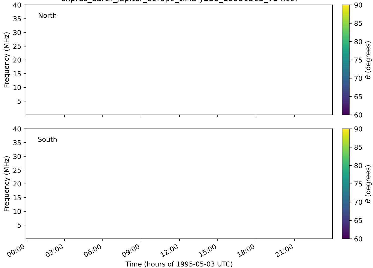
expres_earth_jupiter_europa_txka-y235_19950503_v14.cdf
