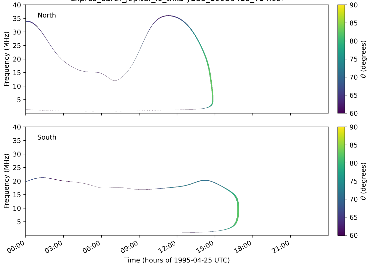
expres_earth_jupiter_io_txka-y235_19950425_v14.cdf
