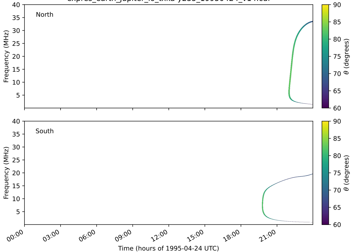
expres_earth_jupiter_io_txka-y235_19950424_v14.cdf
