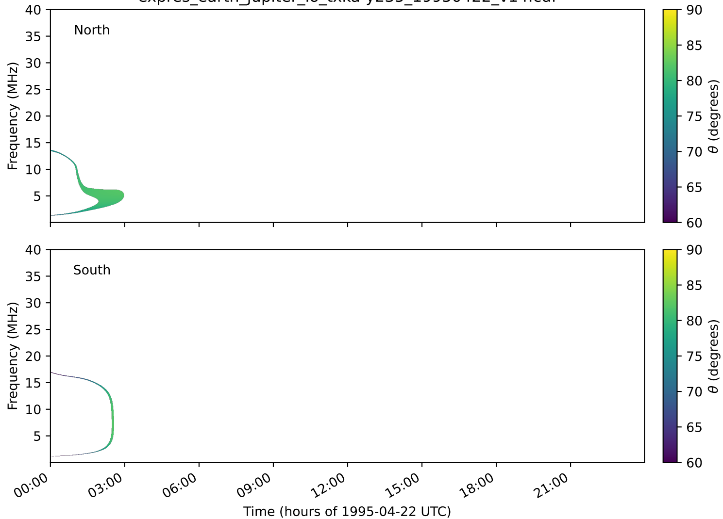
expres_earth_jupiter_io_txka-y235_19950422_v14.cdf
