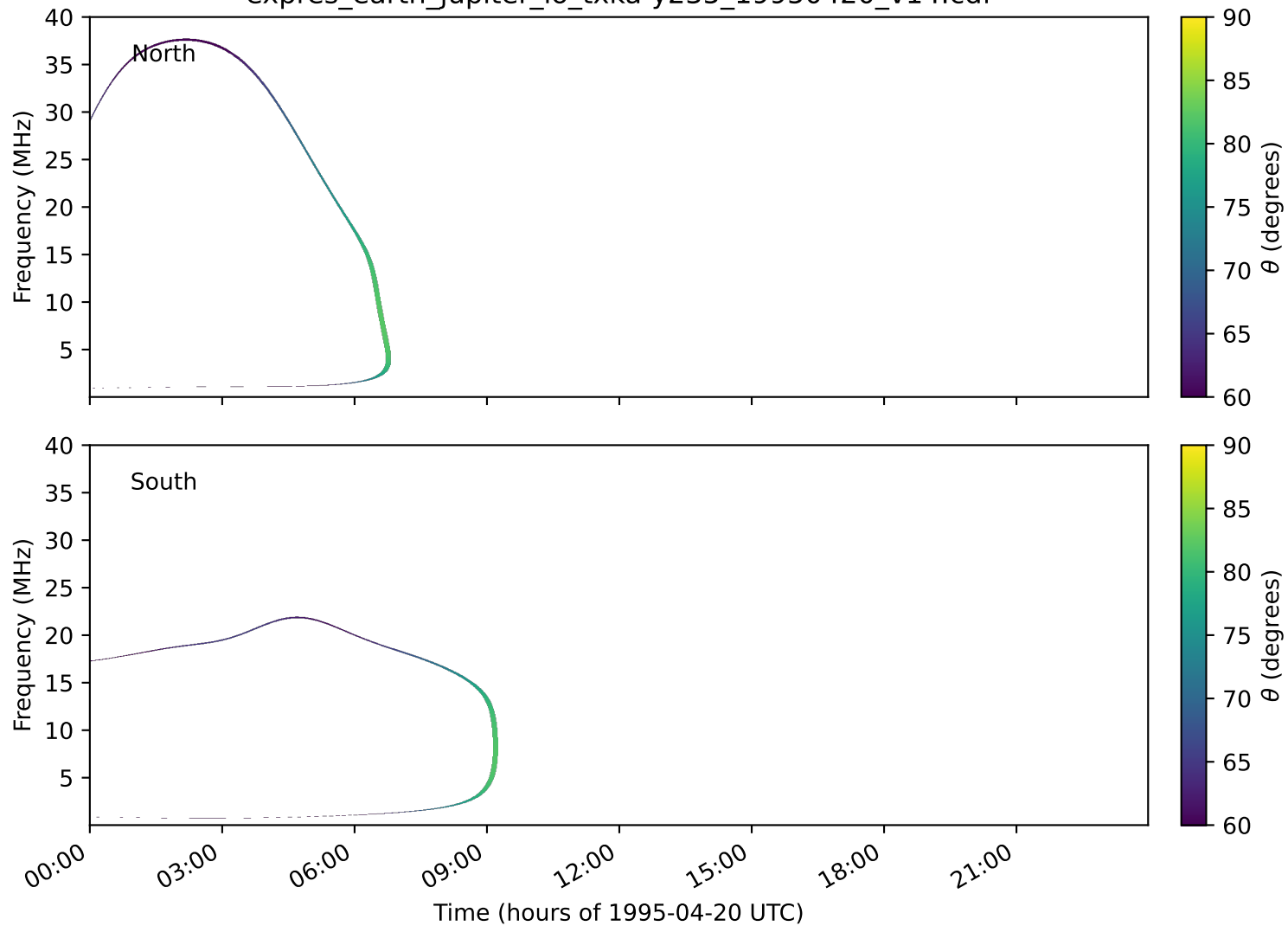
expres_earth_jupiter_io_txka-y235_19950420_v14.cdf
