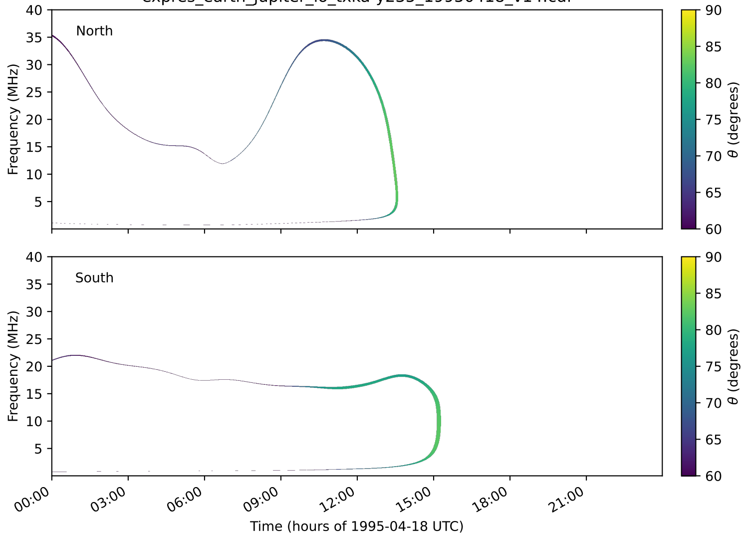
expres_earth_jupiter_io_txka-y235_19950418_v14.cdf
