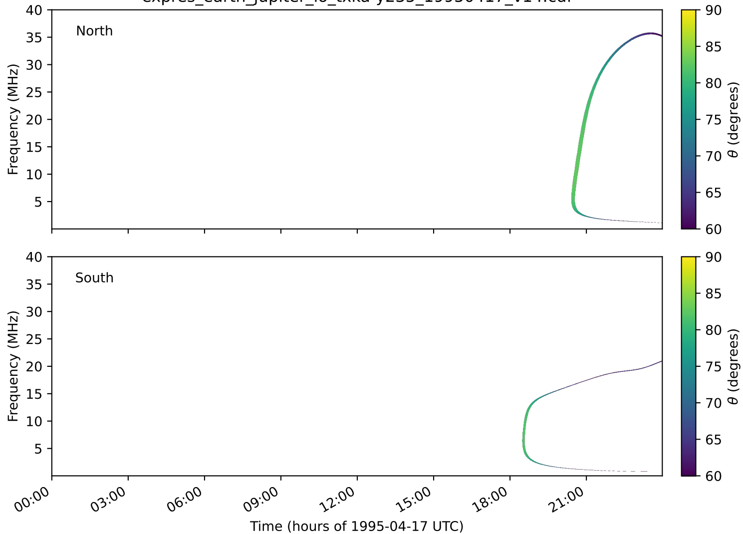
expres_earth_jupiter_io_txka-y235_19950417_v14.cdf
