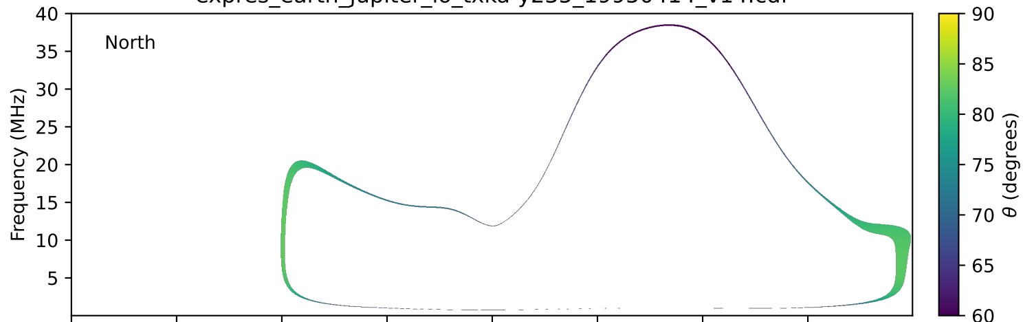
expres_earth_jupiter_io_txka-y235_19950414_v14.cdf
