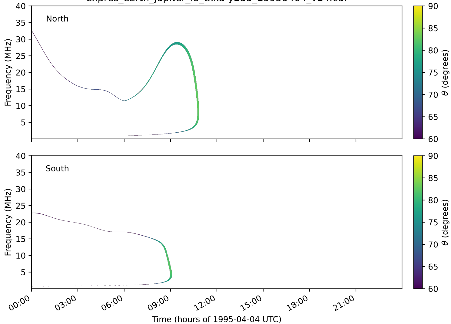
expres_earth_jupiter_io_txka-y235_19950404_v14.cdf
