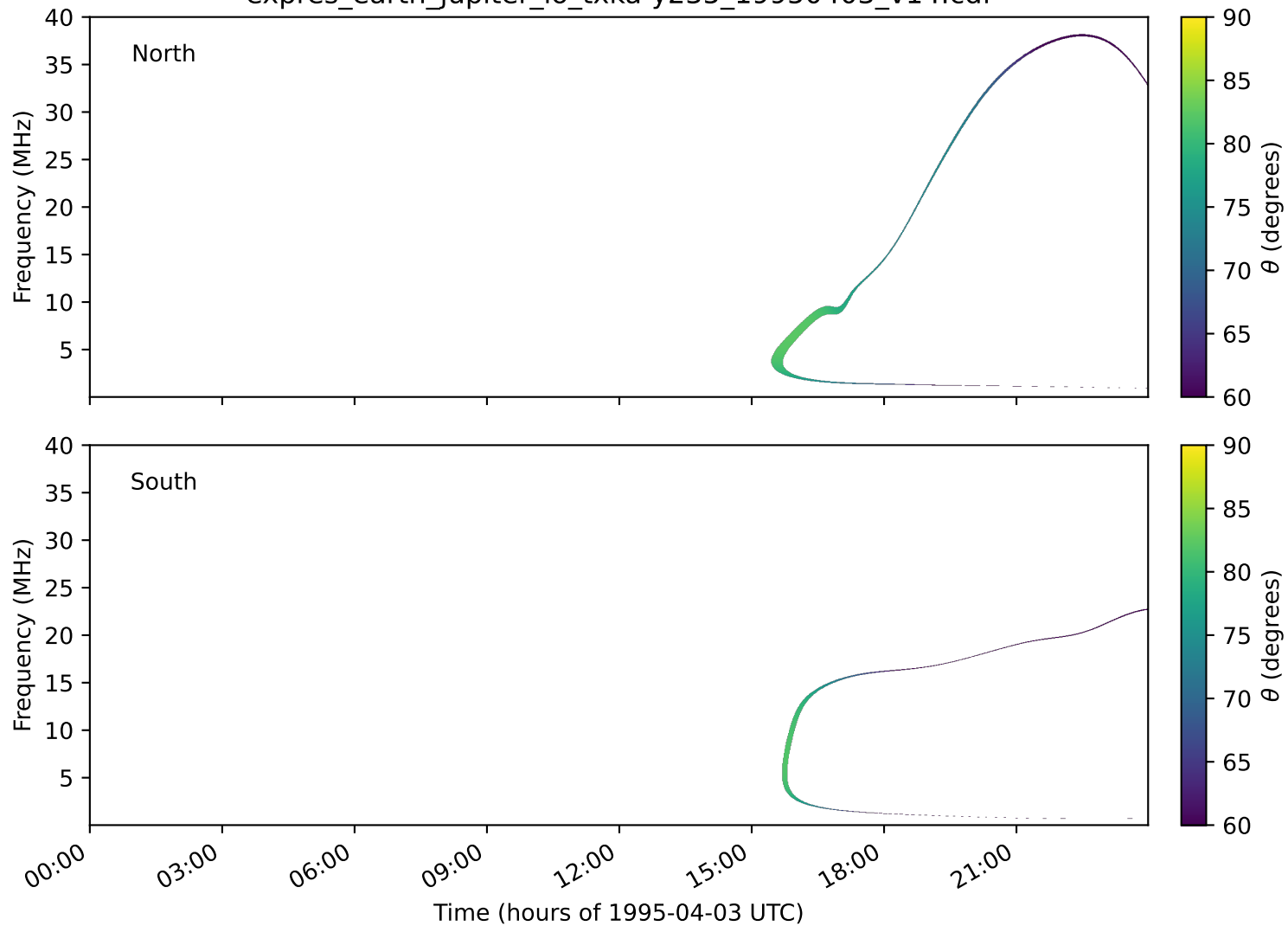
expres_earth_jupiter_io_txka-y235_19950403_v14.cdf
