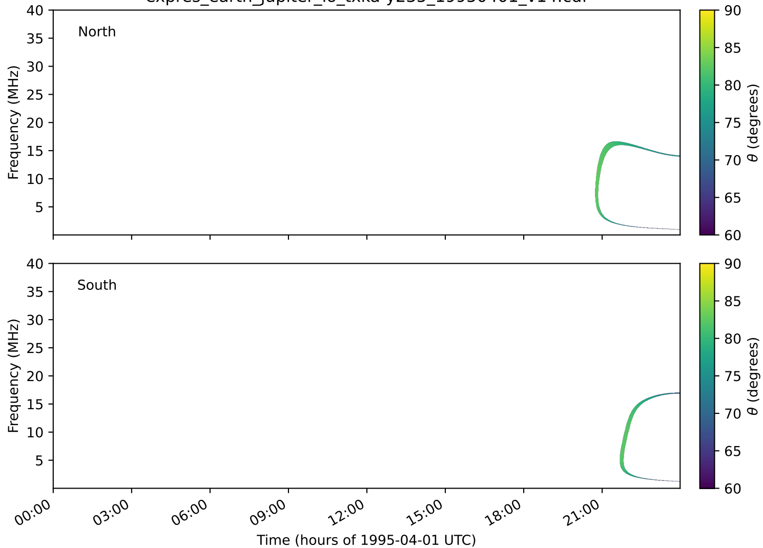
expres_earth_jupiter_io_txka-y235_19950401_v14.cdf
