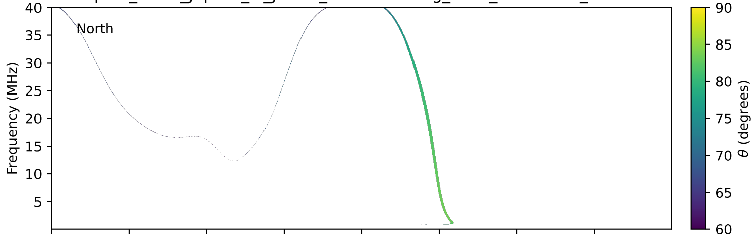
expres_earth_jupiter_io_jrm33_lossc-wid1deg_3kev_19950425_v11.cdf
