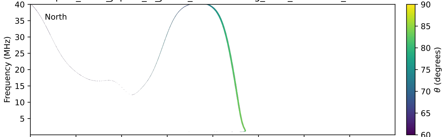
expres_earth_jupiter_io_jrm33_lossc-wid1deg_3kev_19950418_v11.cdf
