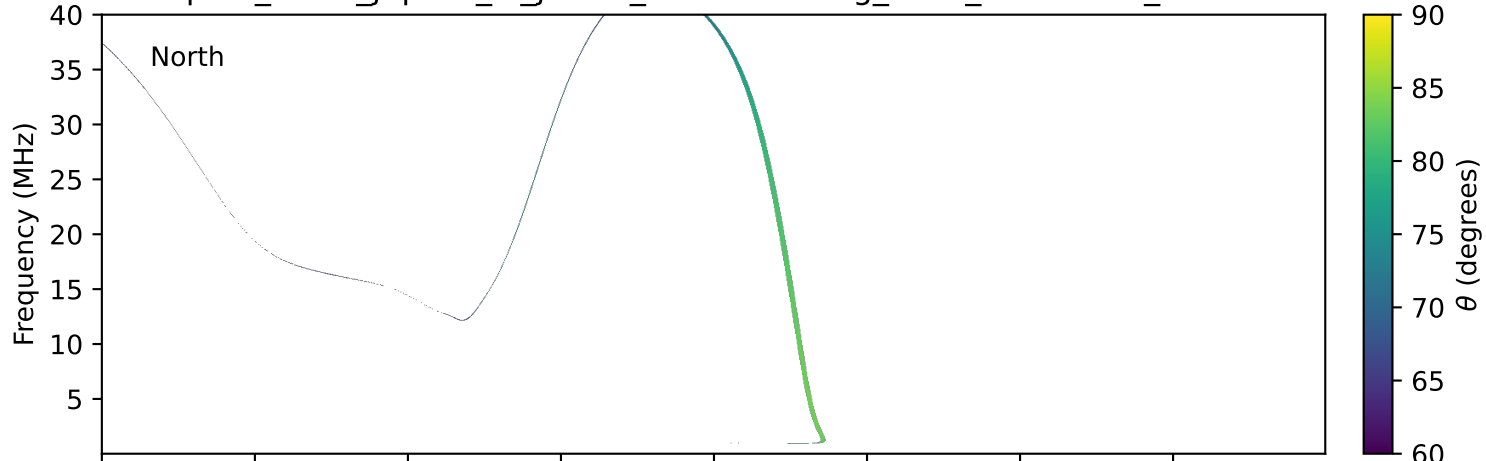
expres_earth_jupiter_io_jrm09_lossc-wid1deg_3kev_19950418_v11.cdf
