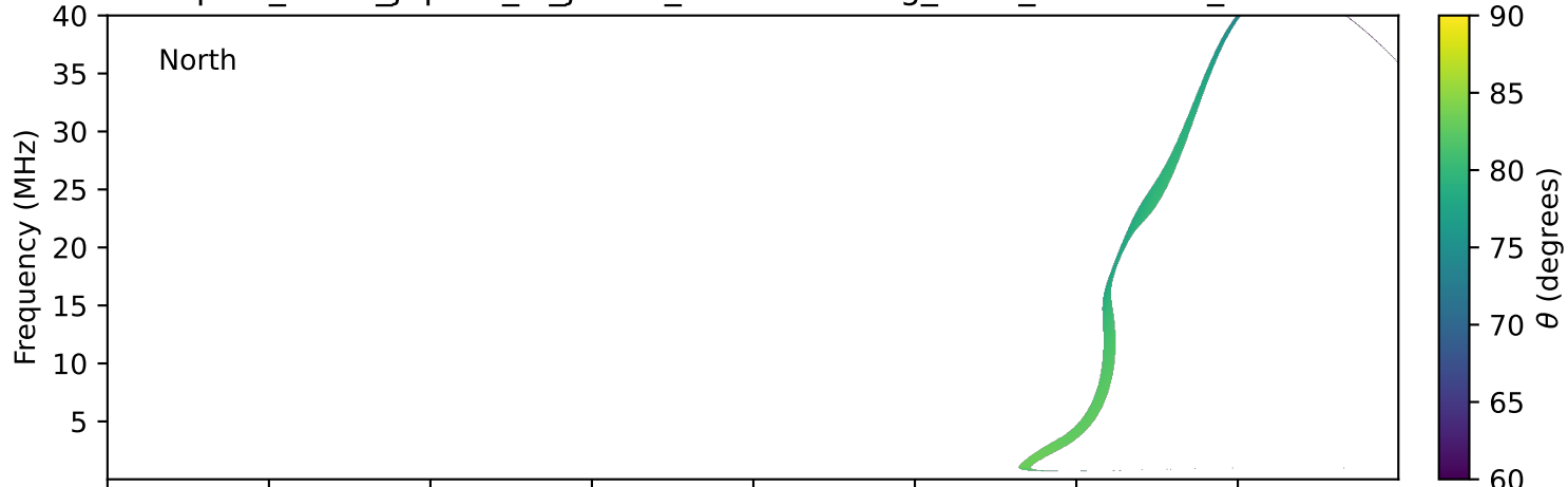
expres_earth_jupiter_io_jrm09_lossc-wid1deg_3kev_19950410_v11.cdf
