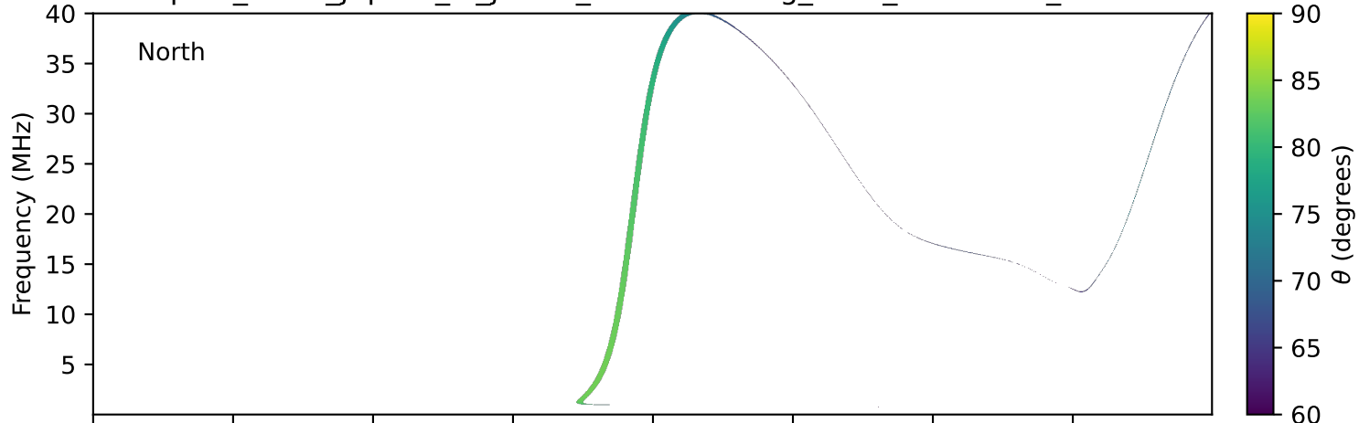
expres_earth_jupiter_io_jrm09_lossc-wid1deg_3kev_19950405_v11.cdf
