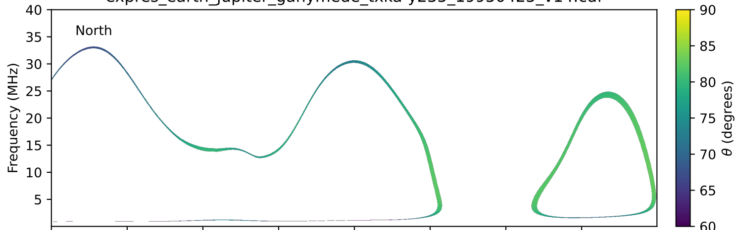
expres_earth_jupiter_ganymede_txka-y235_19950425_v14.cdf
