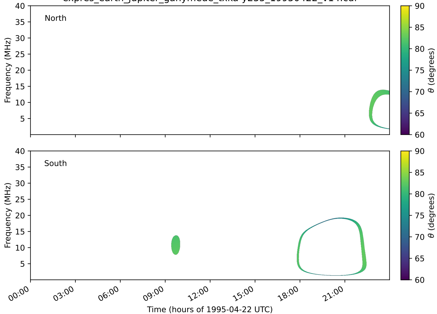
expres_earth_jupiter_ganymede_txka-y235_19950422_v14.cdf
